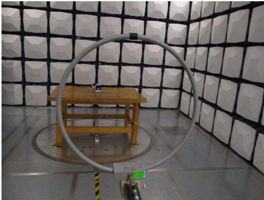
Radiated Emission-Adapter supply View (9 kHz~30 MHz)
