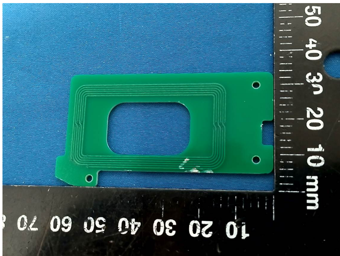
Loop Antenna(13.56MHz)
