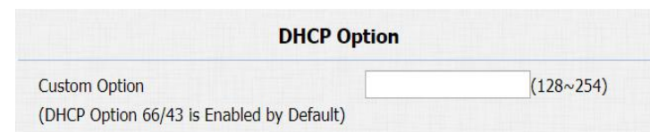
Figure 4.5.4 DHCP Option
