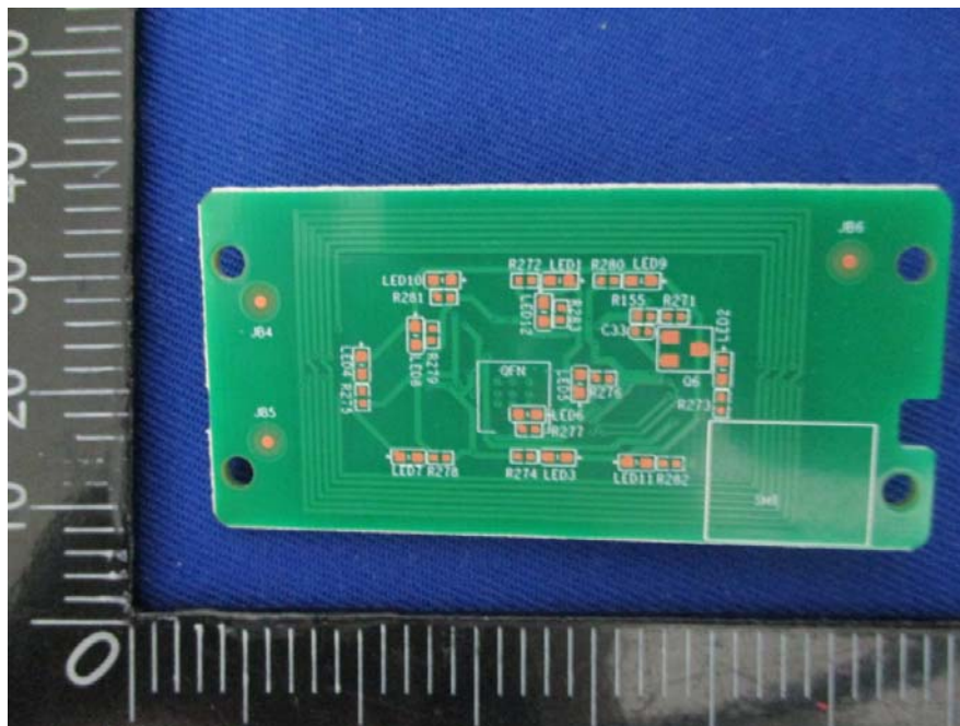
EUT – 13.56MHz Ant View
