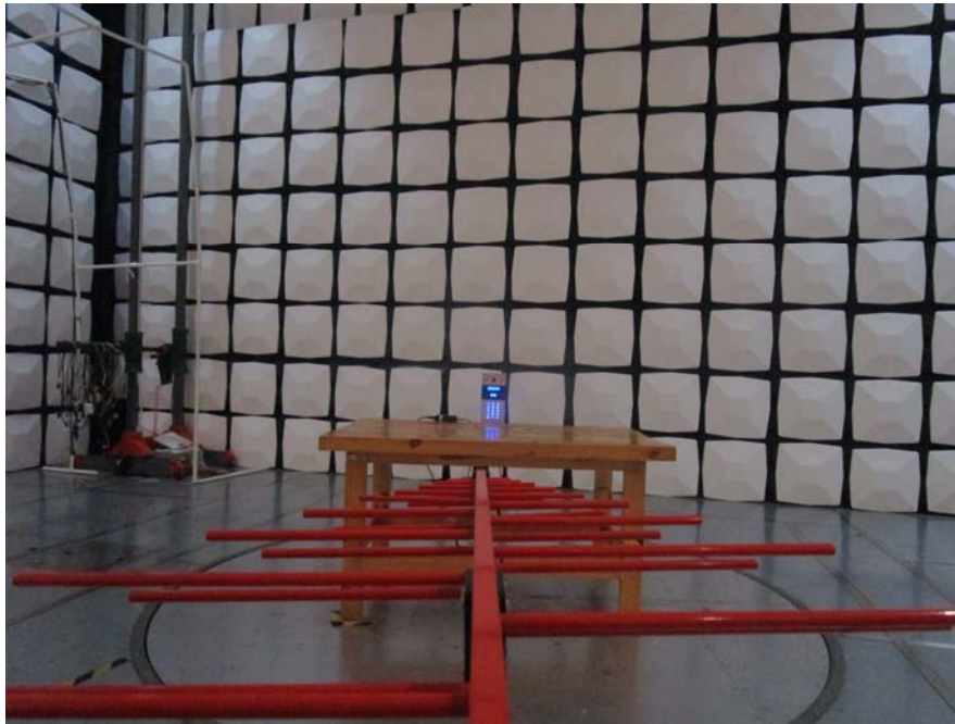
Radiated Emission- Front View(PoE Power Supply)
