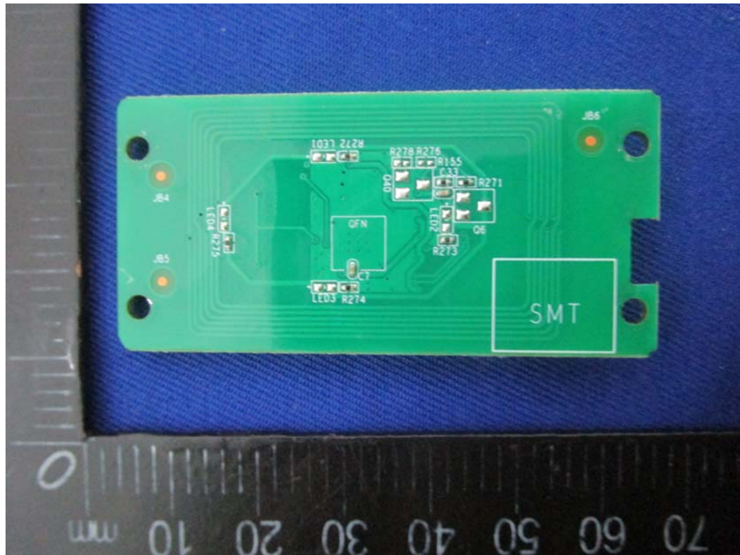
13.56 MHz Antenna Board
