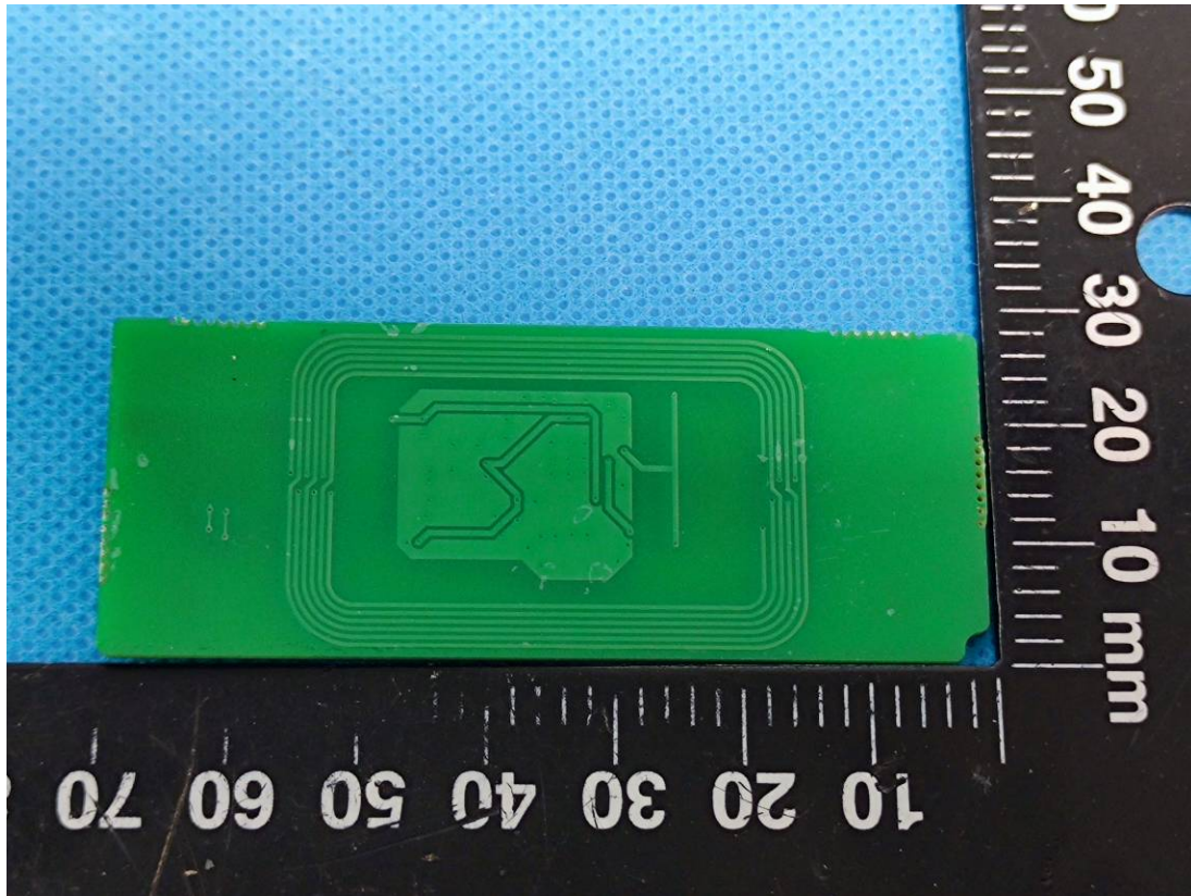
125kHz Antenna
