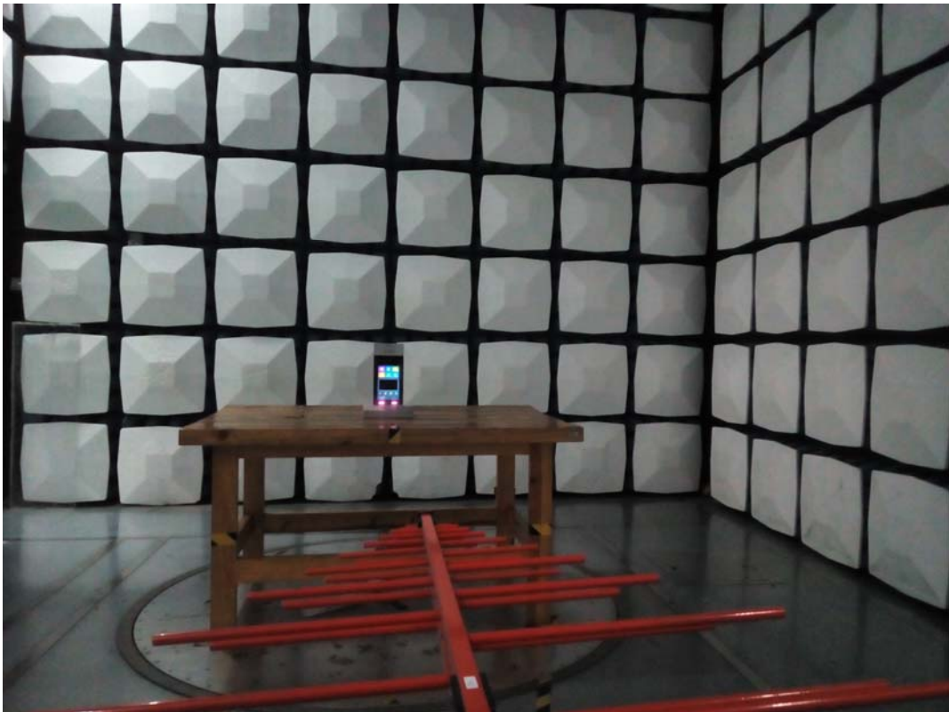
Radiated Emission Below 1GHz 30M-1G View
