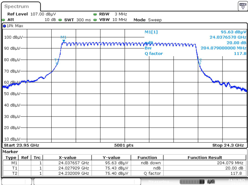
20 dB Bandwidth
