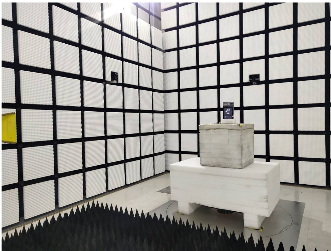
Radiated Emission Above 1GHz View-POE
