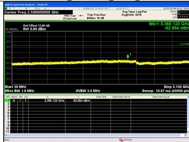
Spurious Emission:30.0~5150 MHz IEEE 802.11ac_Channel 62_40MHz_Antenna 0
