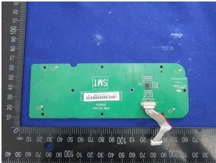
EUT – Keyboard PCB Top View
