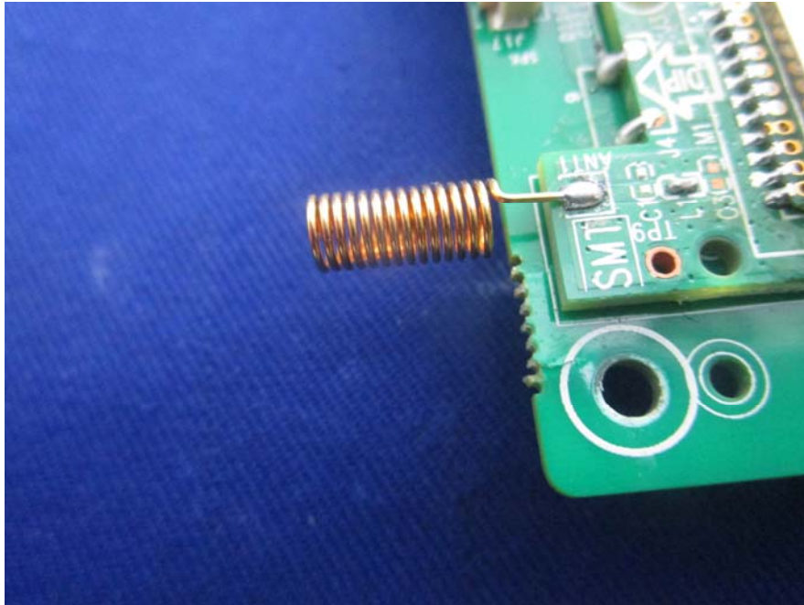
EUT – 434MHz Antenna View
