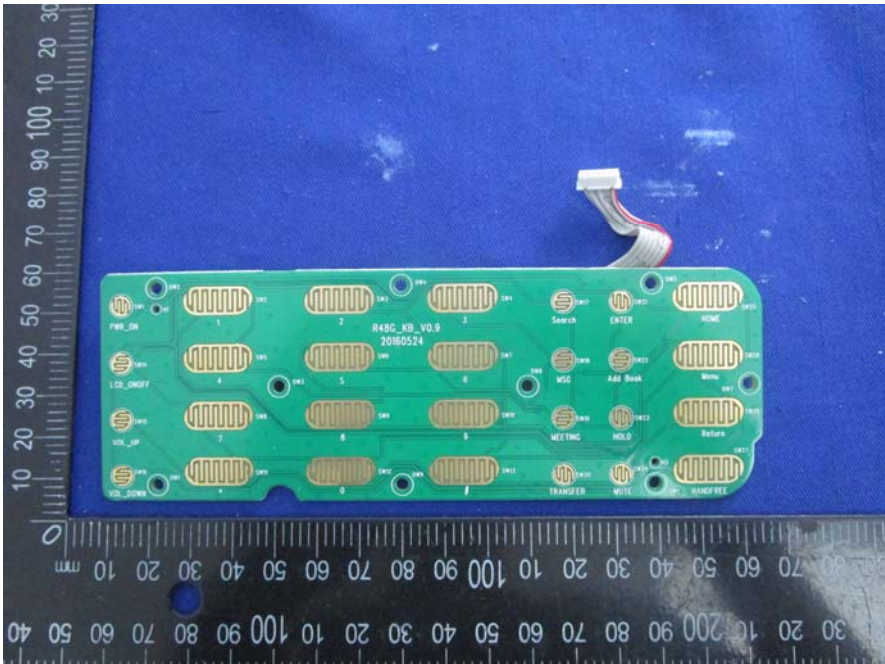
EUT – Keyboard PCB Bottom View
