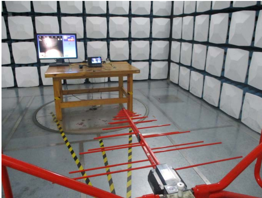
Radiated Emission View (Below 1GHz)-Adapter
