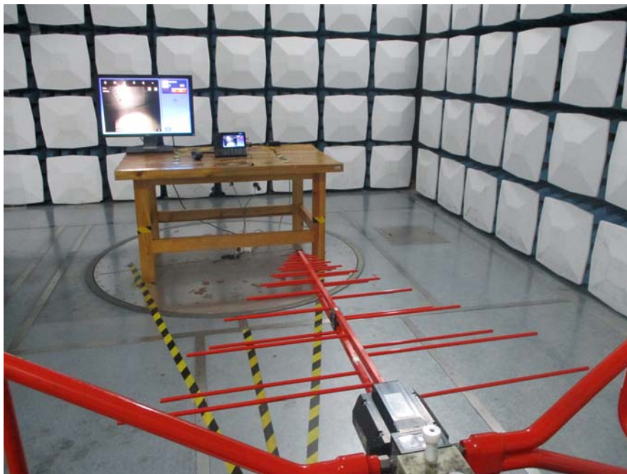
Radiated Emission View (Below 1GHz)-PoE
