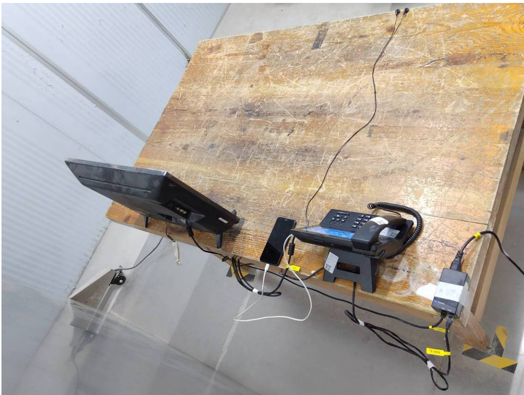
Conducted Emissions Side View- POE
