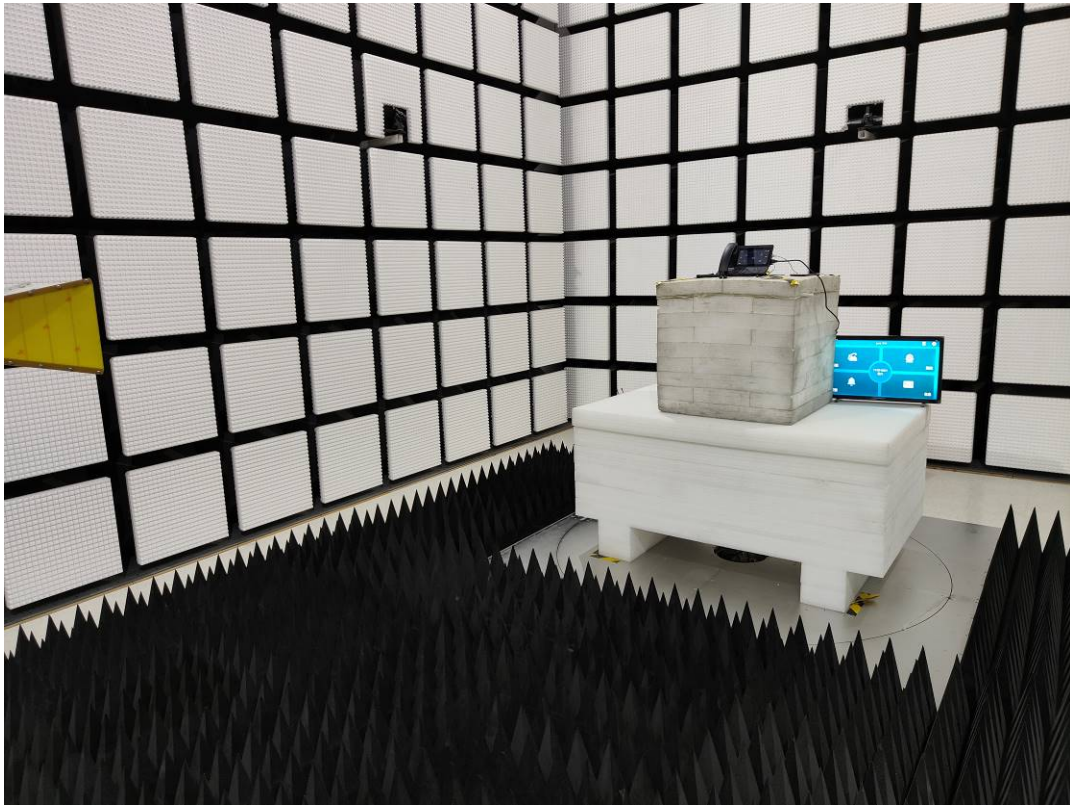
Radiated Emissions Above 1G front View -Adapter
