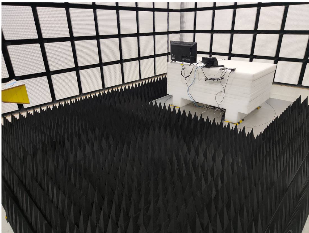
Radiated Emissions Above 1G rear View-POE Adapter
