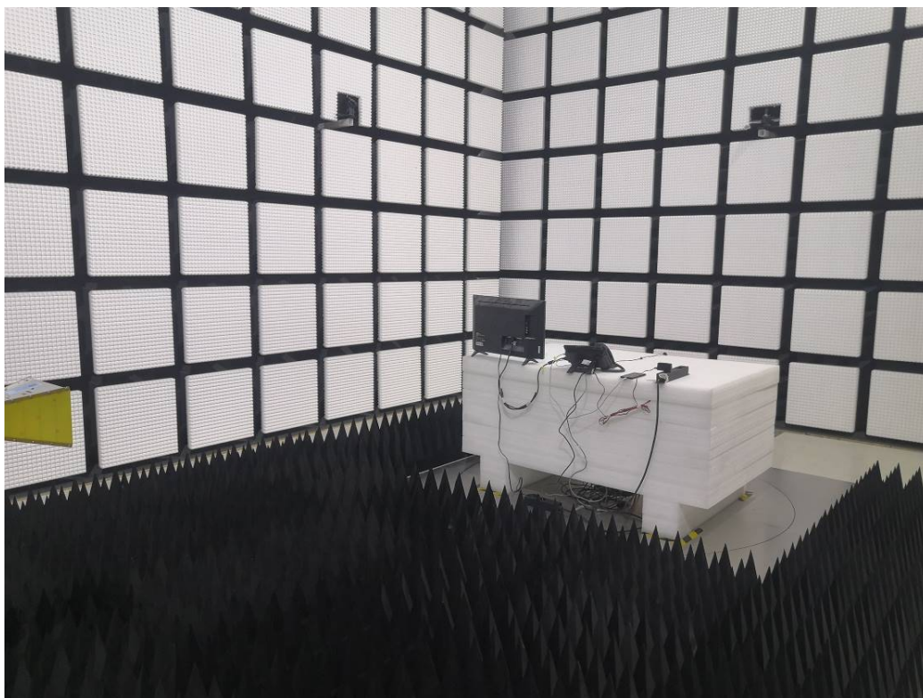
Radiated Emissions Above 1G rear View- AC/DC Adapter
