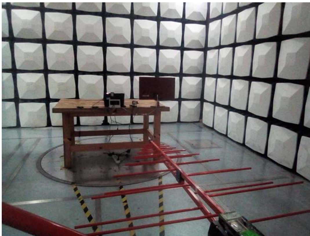
Radiated Emission Below 1GHz Rear View Adapter
