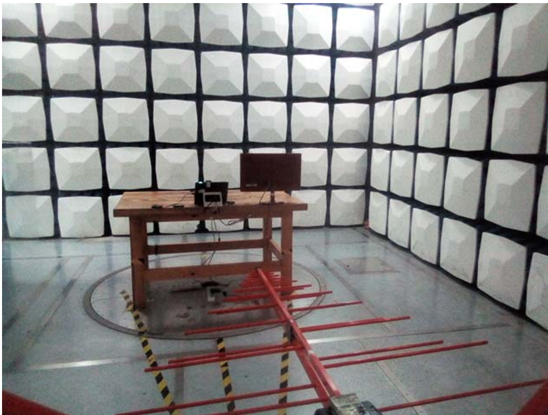
Radiated Emission Below 1GHz Rear View POE
