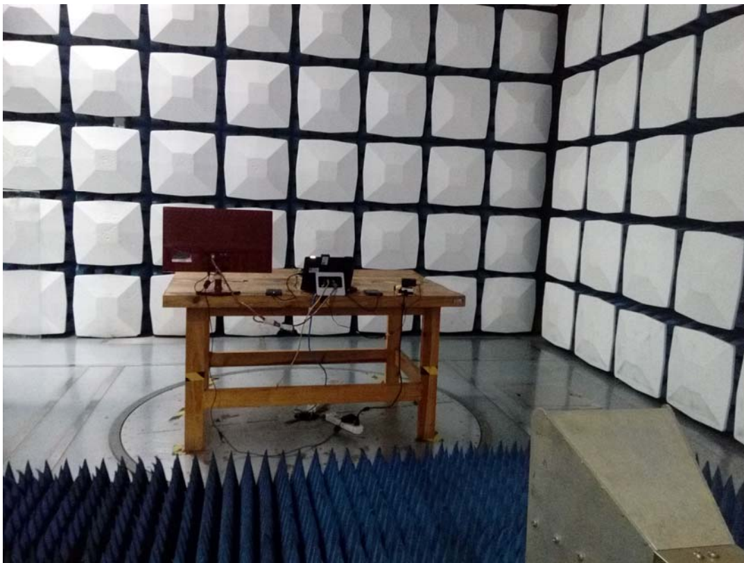
Radiated Emission Above 1GHz Rear View Adapter
