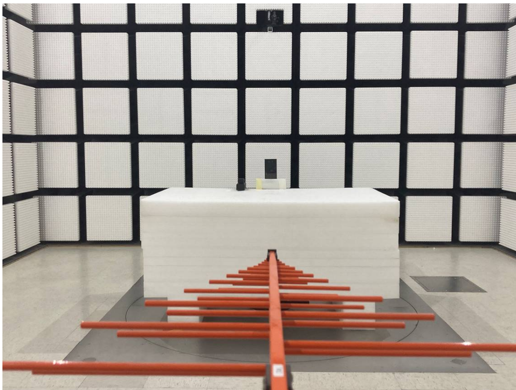
Radiated Emission Below 1GHz View-Adapter Power Mode
