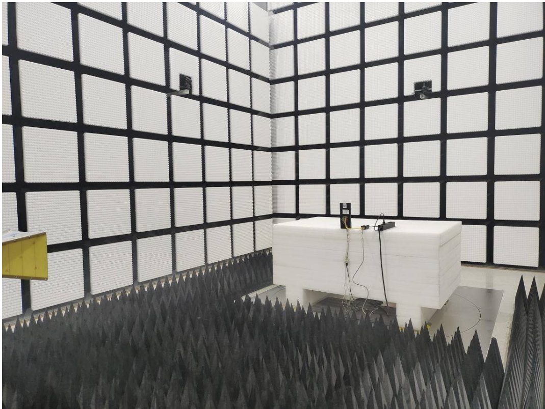
Radiated Emission Above 1GHz View-PoE Power Mode
