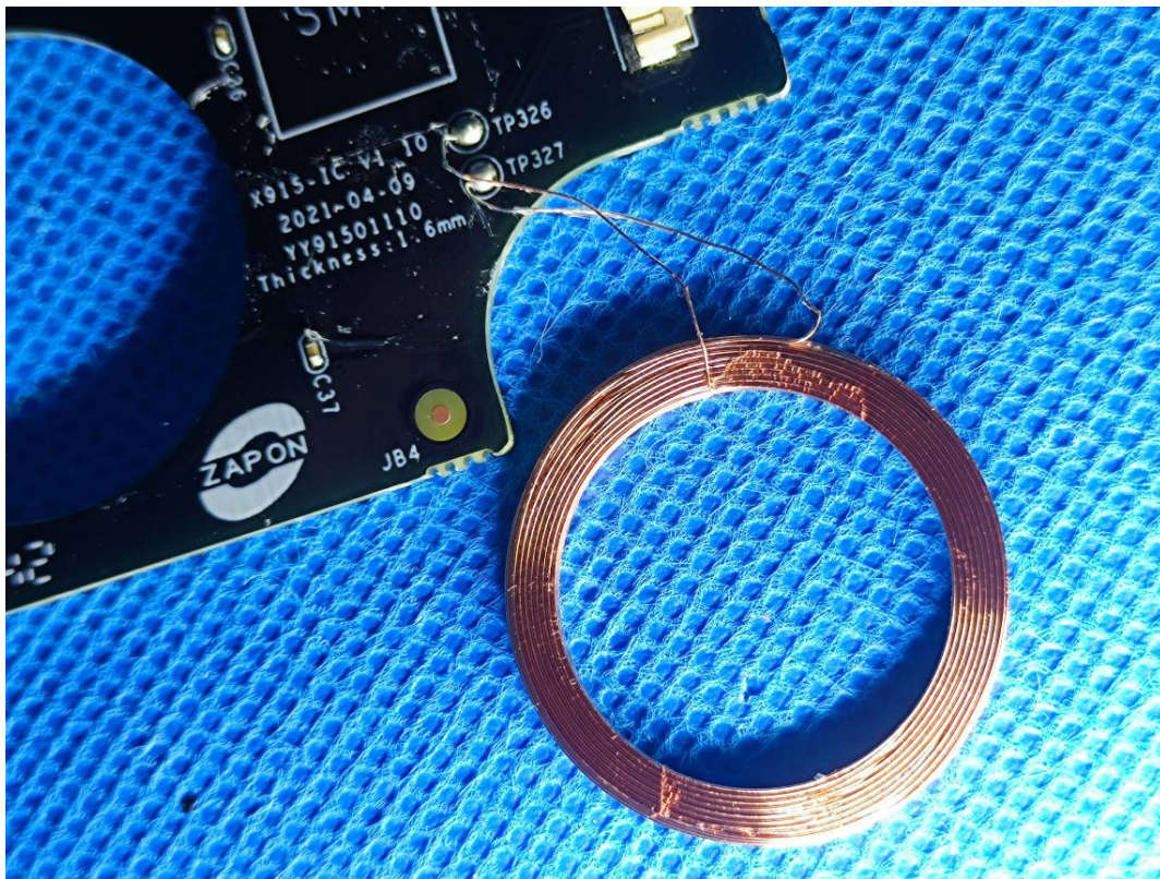
125kHz Antenna
