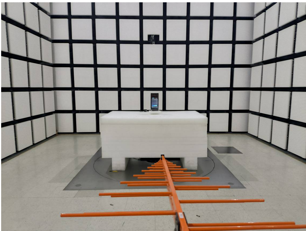
Radiated Emission Below 1GHz View-Powered byPoE
