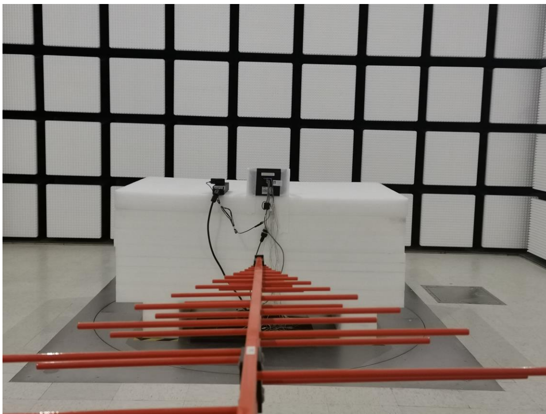
Radiated Emission Below 1G rear View- Adapter Power Mode
