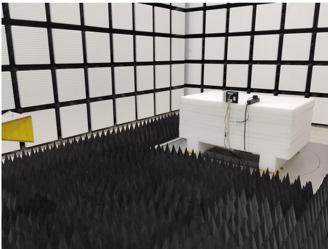
Radiated Emission Above 1GHz View- Adapter Power Mode
