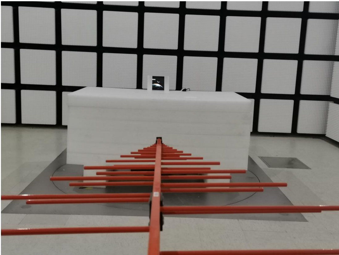
Radiated Emission Below 1G rear View- PoE Power Mode
