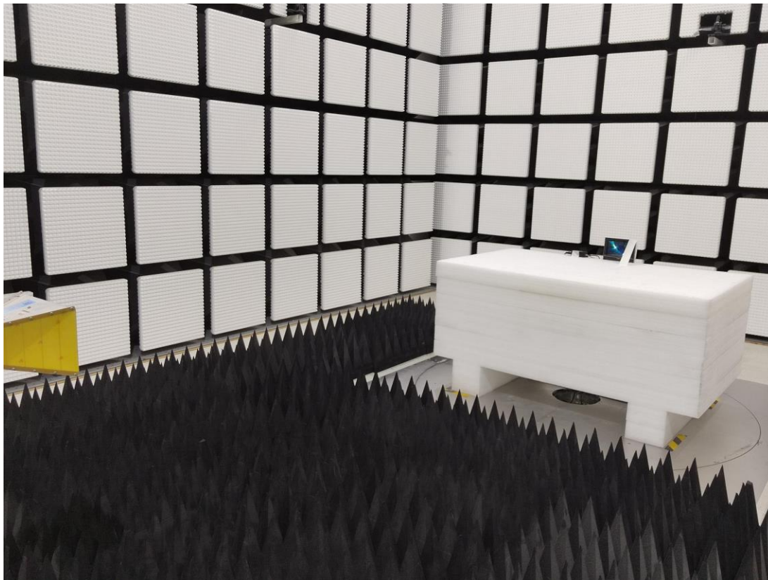
Radiated Emission Above 1GHz View- PoE Power Mode
