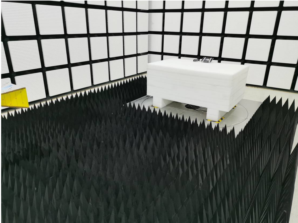
Radiated Emissions Above 1G rear View-PoE
