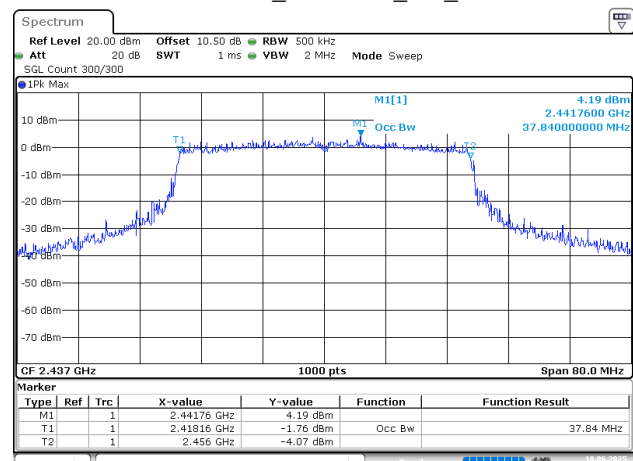
802.11ax40_2437MHz_RU_Full
