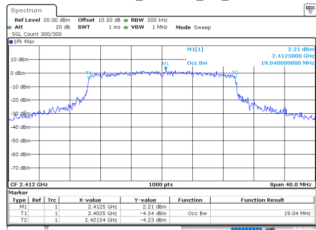
802.11ax20_2412MHz_RU_Full
