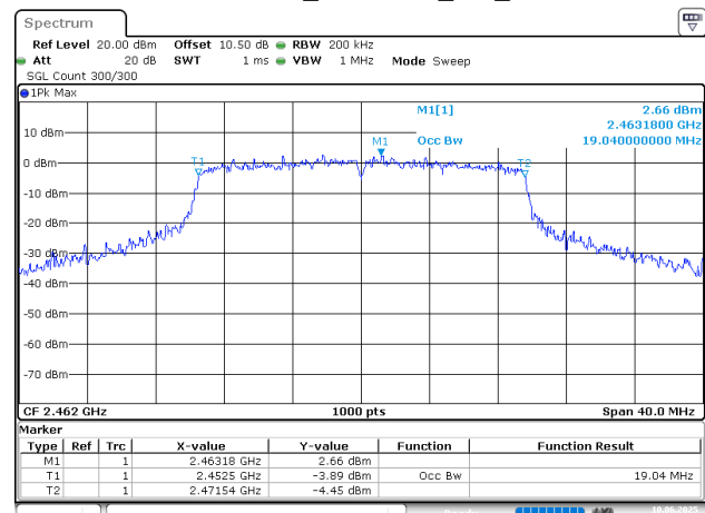
802.11ax20_2462MHz_RU_Full
