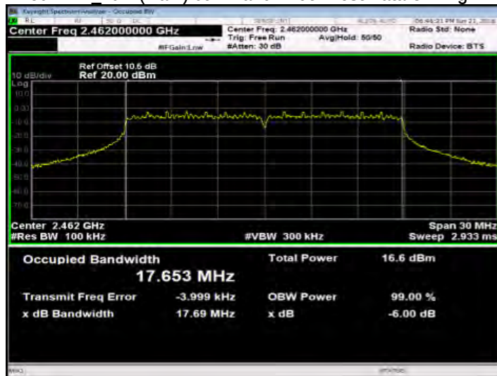
802.11n_20M (Main) 6dB Band Width Test Data CH-High
