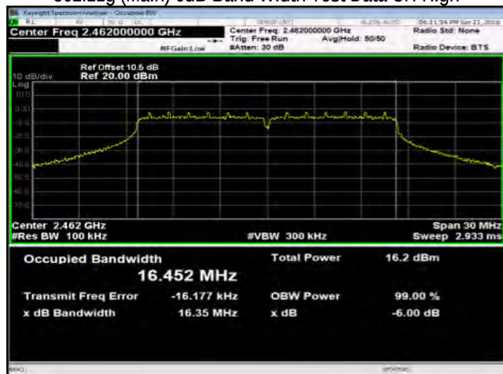
802.11g (Main) 6dB Band Width Test Data CH-High
