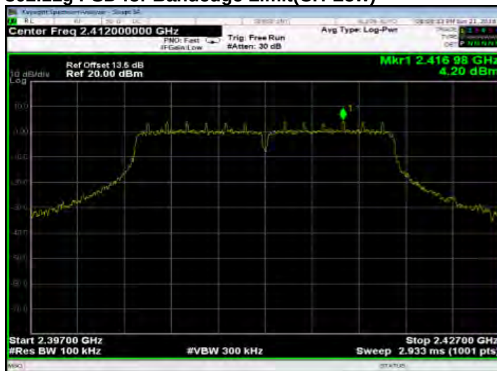
802.11g PSD for Bandedge Limit(CH-Low)
