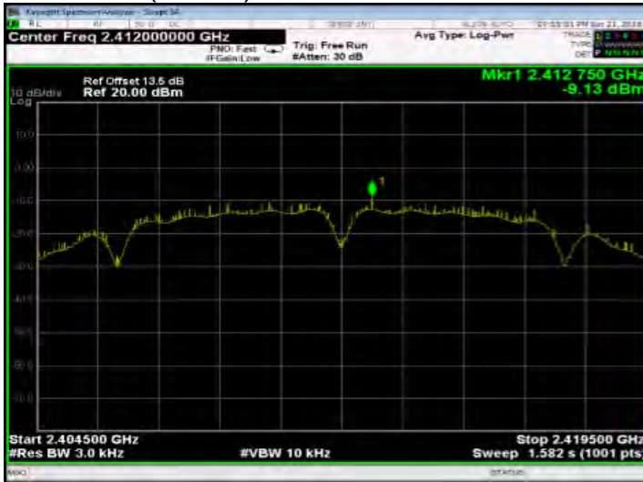
802.11b PSD (CH-Mid)
