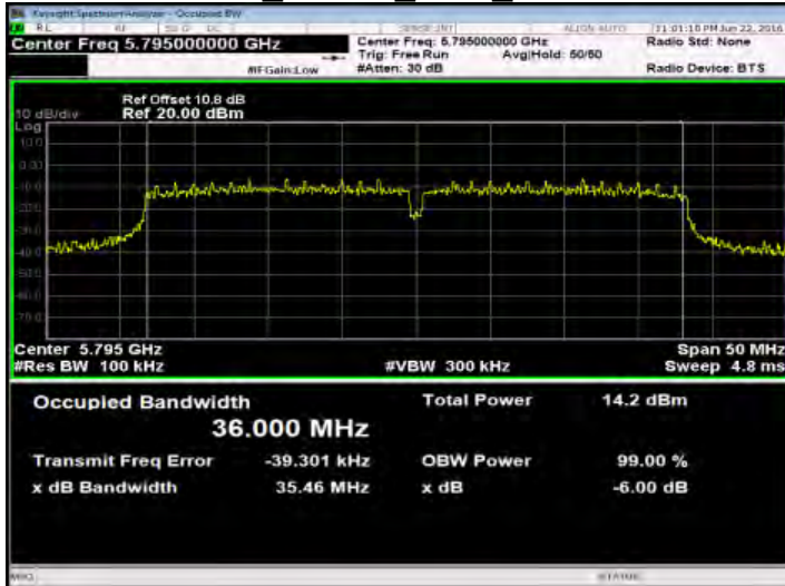
802.11n 40MHz Main 5795MHz
