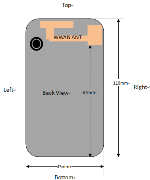
Fig.14.1 EUT Antenna Locations
