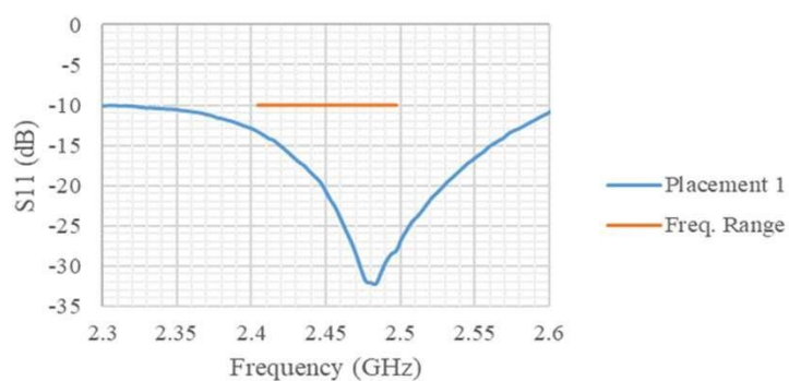
S11 of Antenna
