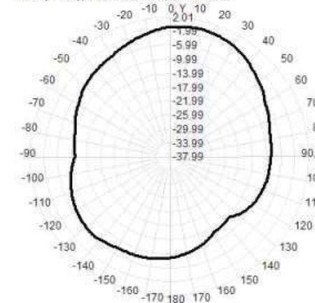
Total(H-XY), Max=-0.24dBi, CirD=13.38
