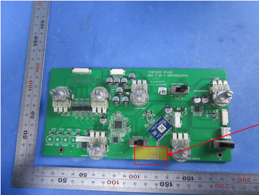
BT Antenna
