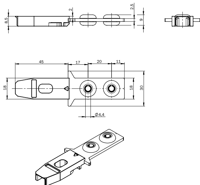
Figure 47: Dimensional drawing of TR110-XAS straight actuator (mm)
