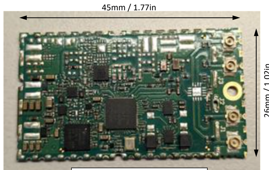
Front side w/o metal cover
