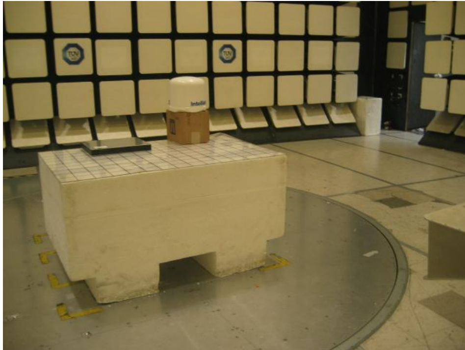
Radiated Spurious Emissions Test Setup (Front View)
