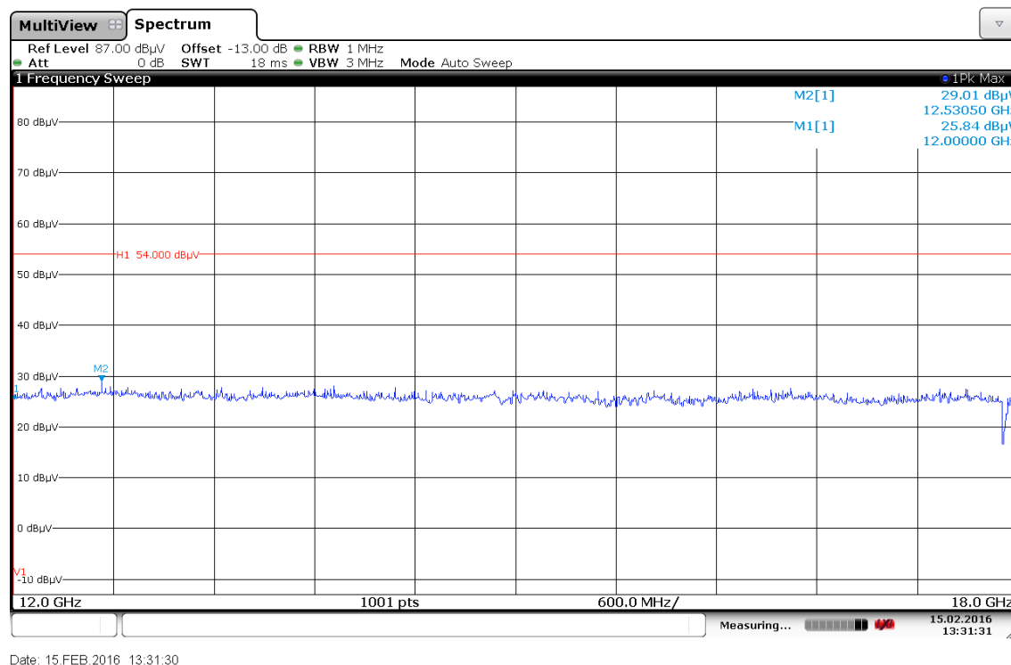
Plot No. 8: 12 GHz to 18 GHz, horizontal/vertical polarization
