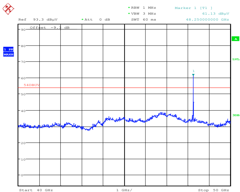
Plot No. 12: 40 GHz to 50 GHz, horizontal / vertical polarization
