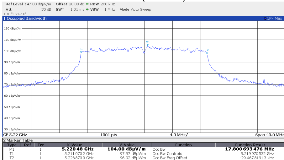
Channel 44 (5220 MHz)
