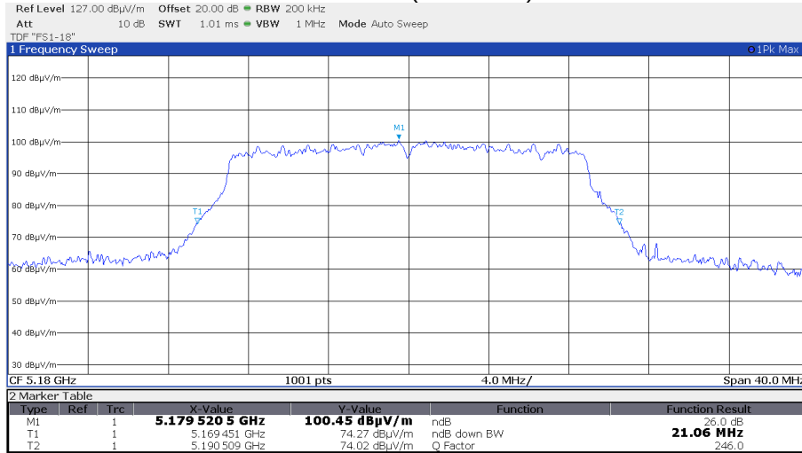
Channel 36 (5180 MHz)
