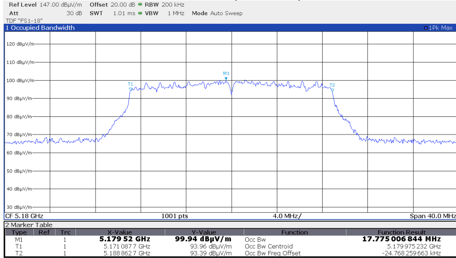
Channel 36 (5180 MHz)
