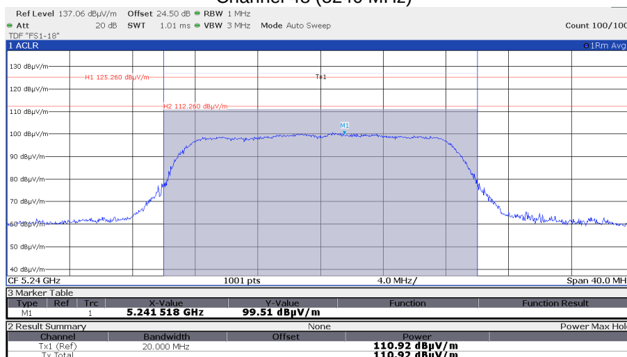
Channel 48 (5240 MHz)
