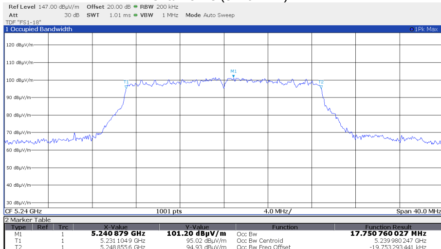
Channel 48 (5240 MHz)
