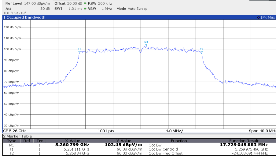
Channel 52 (5260 MHz)
