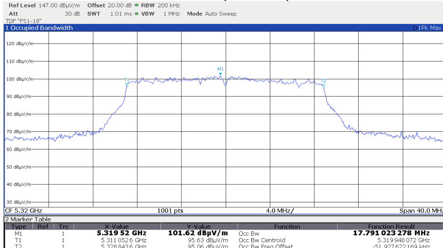
Channel 64 (5320 MHz)
