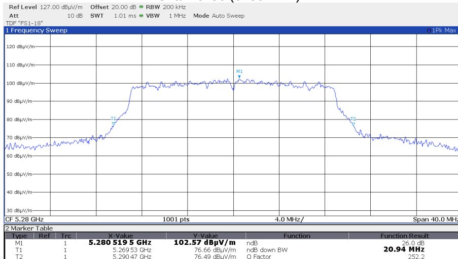
Channel 56 (5280 MHz)
