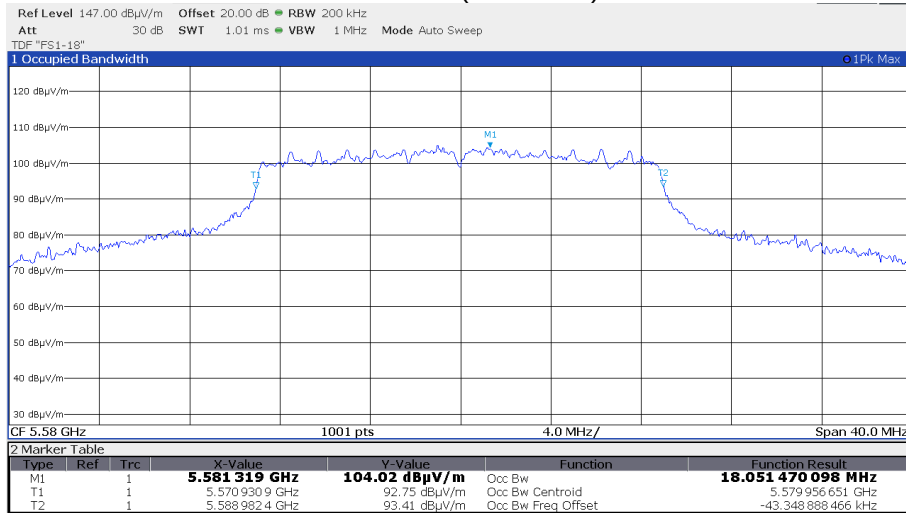
Channel 116 (5580 MHz)
