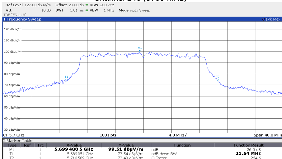
Channel 140 (5700 MHz)
