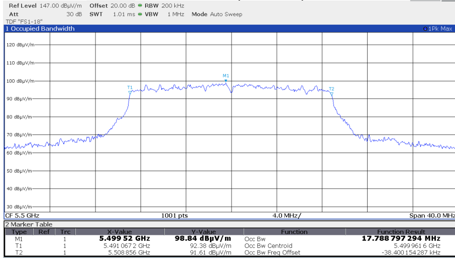
Channel 100 (5500 MHz)
