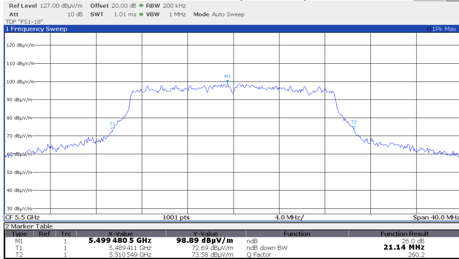
Channel 100 (5500 MHz)
