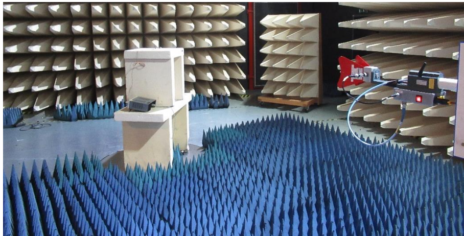
Anechoic chamber
