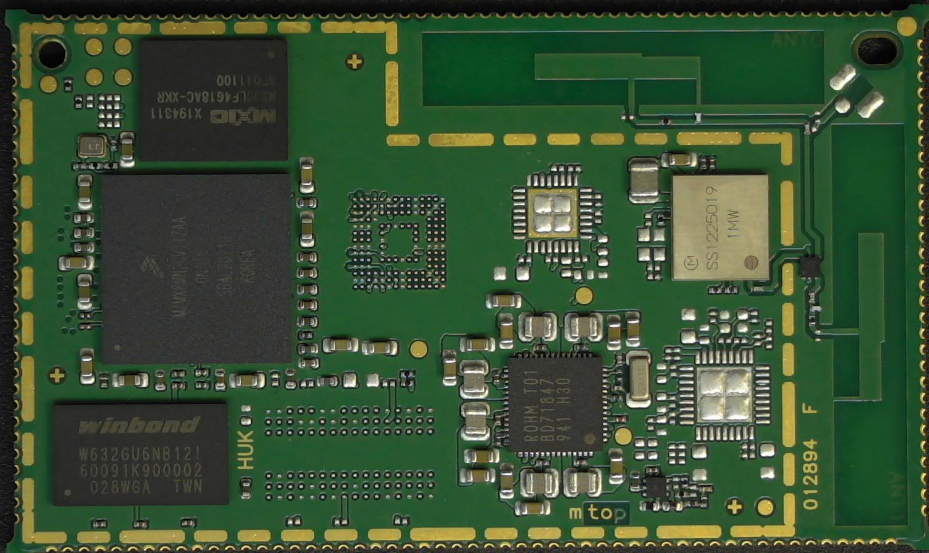
S2_012894-F_V02_top
