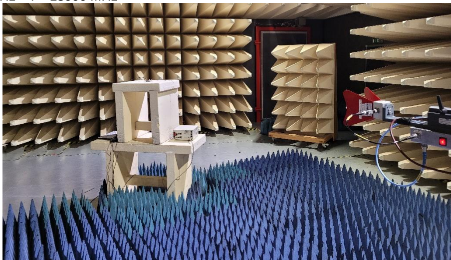
Anechoic chamber
