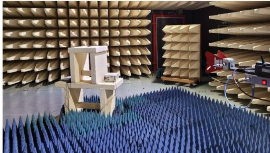
Test Setup 1000 \text{ MHz} < f < 18000 \text{ MHz}
