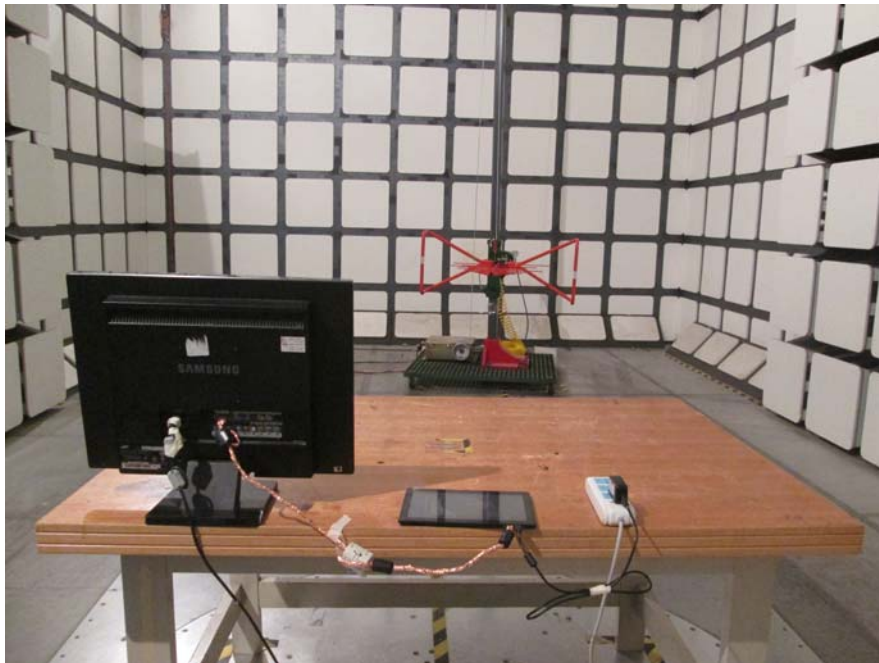
Radiated Emissions – Rear View (Below 1 GHz, HDMI & Charging Mode)
