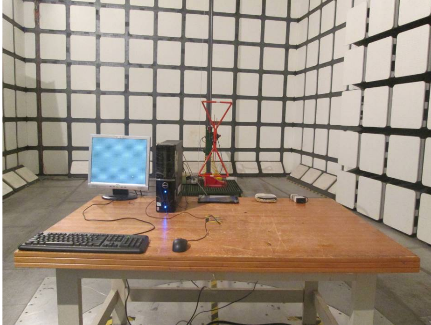
Radiated Emissions – Front View (Below 1 GHz, Downloading Mode)
