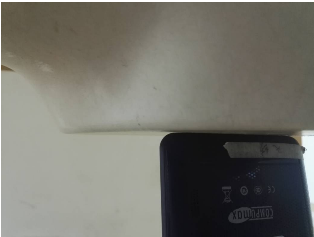
Body-worn Bottom Setup Photo (0mm)
