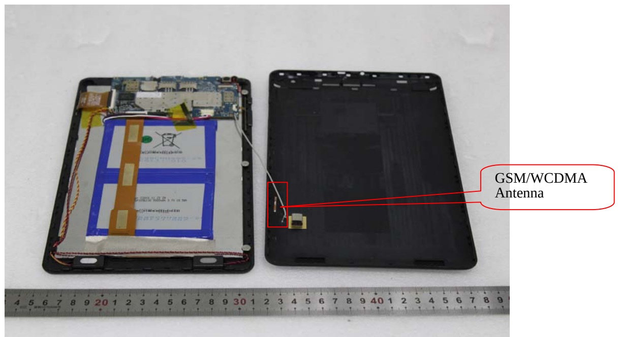
EUT – Cover off View 2
