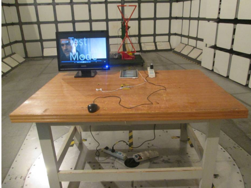
Radiated Emissions – Front View (Below 1 GHz- HDMI Mode)
