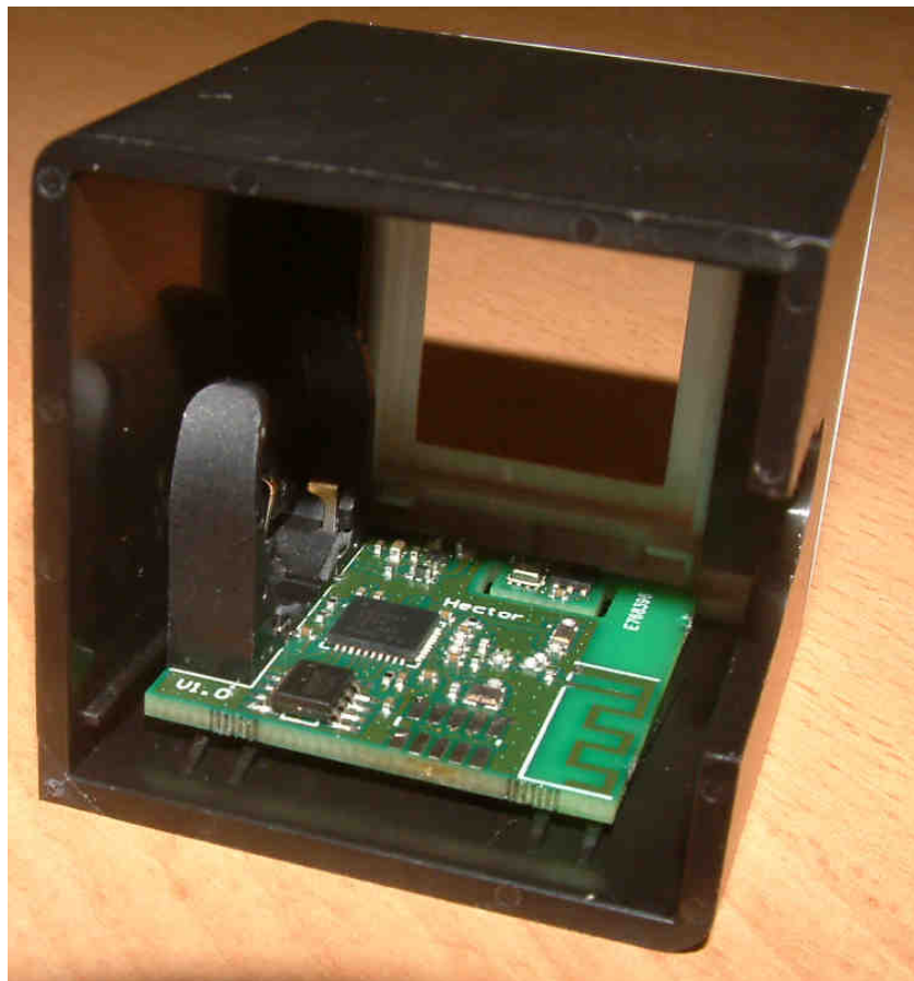
PCB placement
