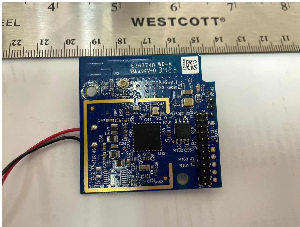
Figure 1. Equipment under Test (Radio module) Frontside
