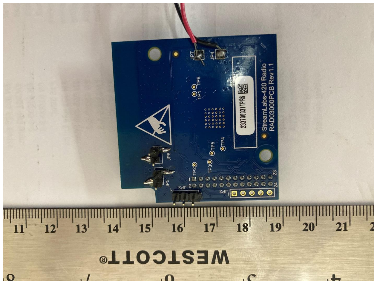
Figure 2. Equipment under Test (Radio module) Backside
