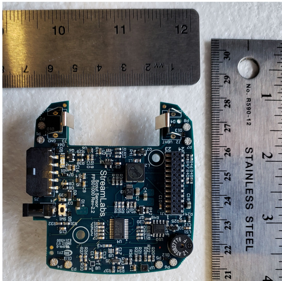
Figure 6. PSB 2 Top
