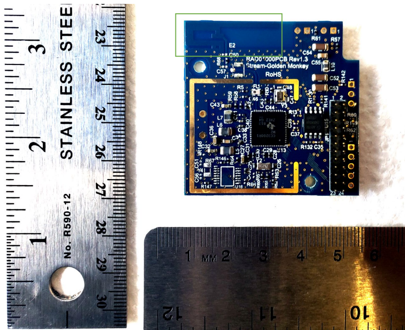
Figure 4. PSB 1 Top
