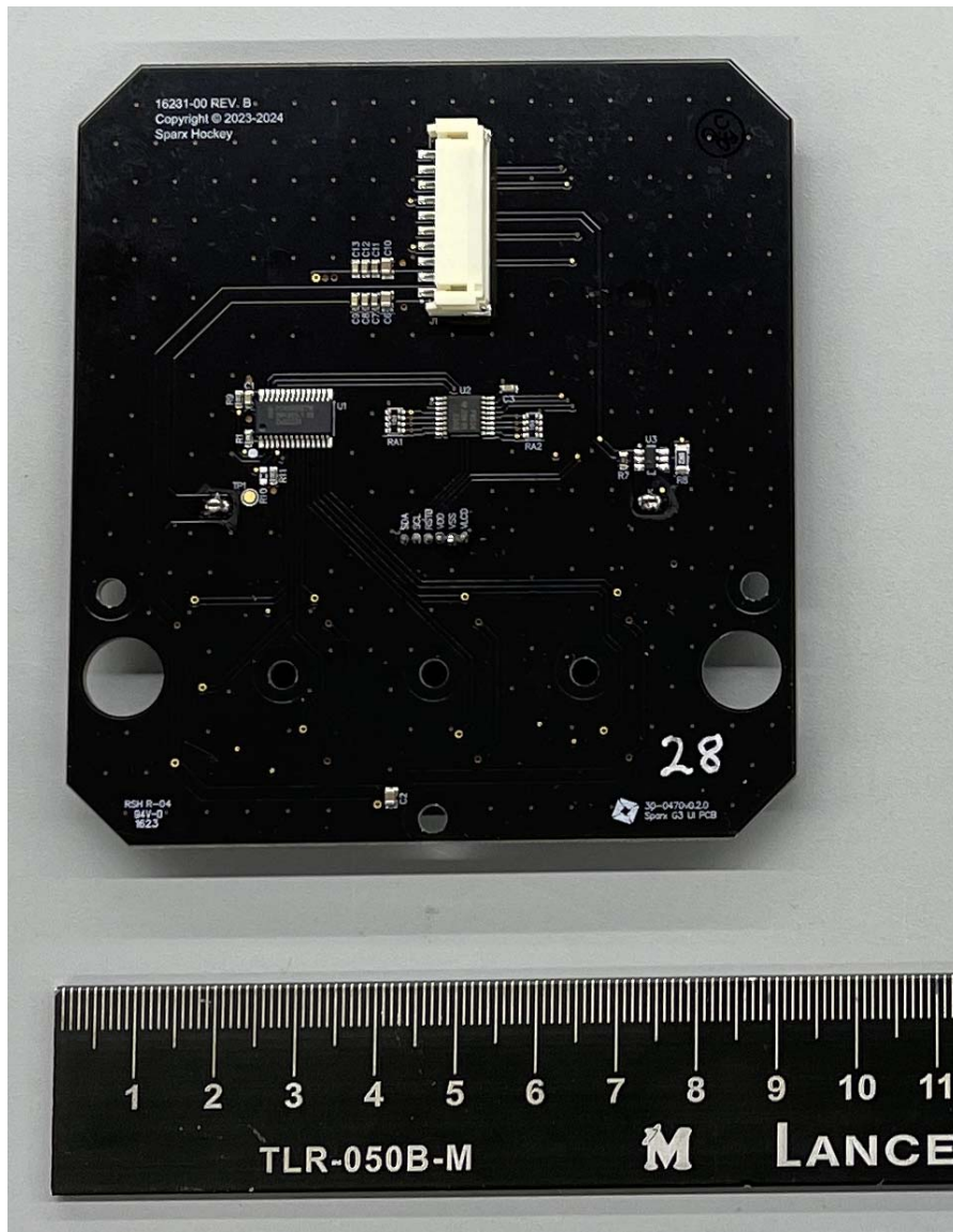
UI PCBA Rear
