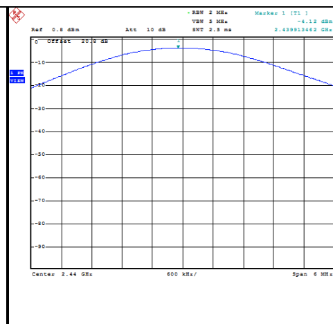
Figure 7.4.2-2: Output Power – Mid Channel
