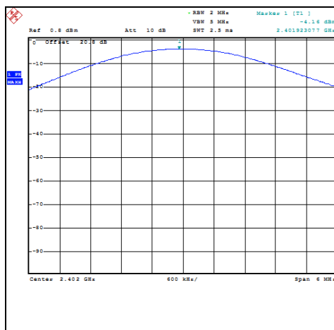
Figure 7.4.2-1: Output Power – Low Channel
