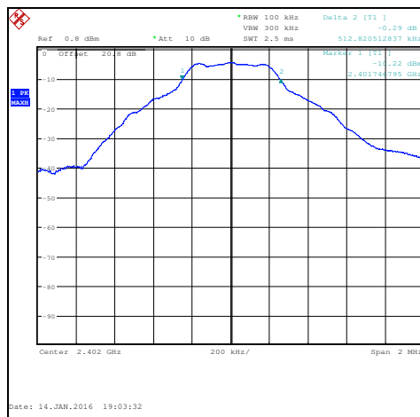
Figure 7.3.2-1: 6dB Bandwidth Low Channel
