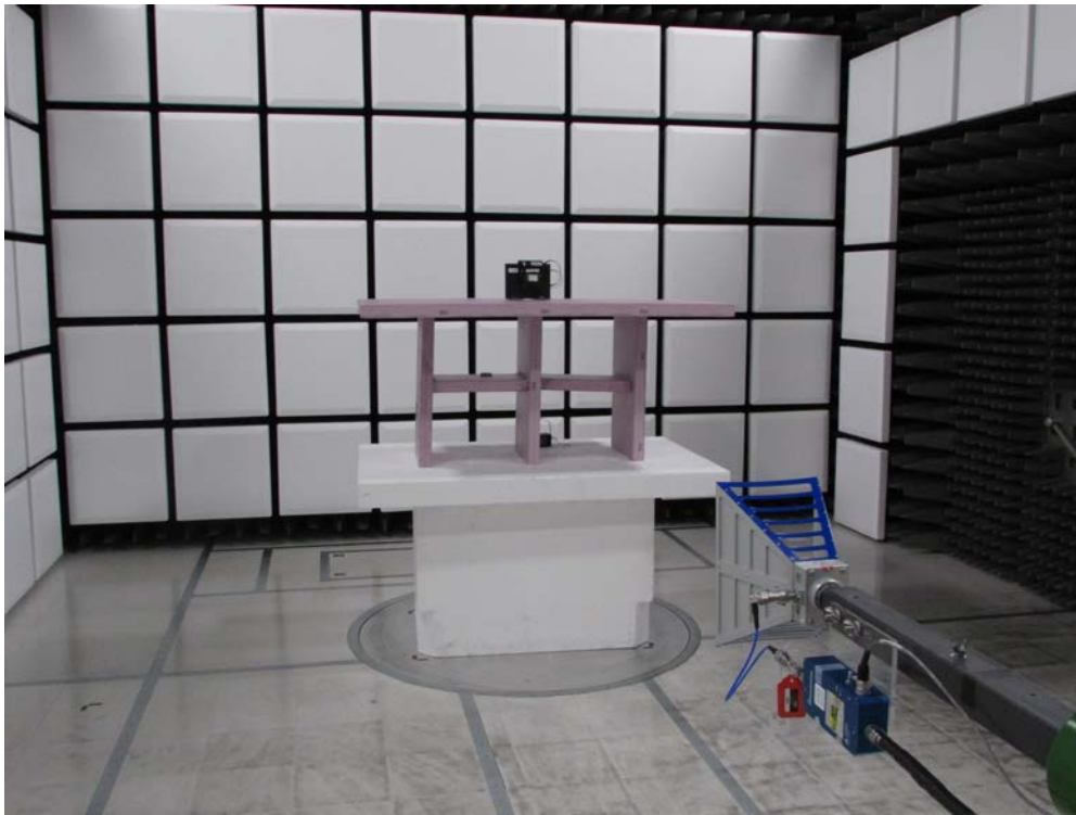
Figure 1: Radiated Emissions Test Set Up – Front View
