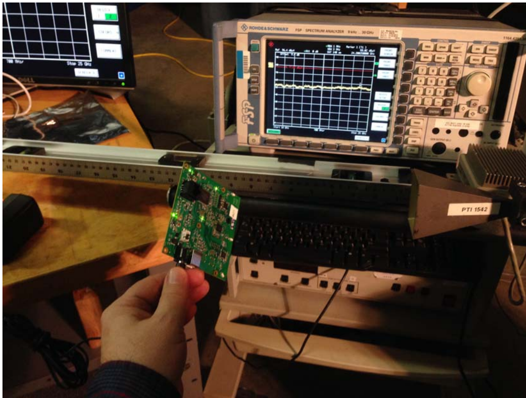
18 to 25 GHz Radiated Pre-Scan
